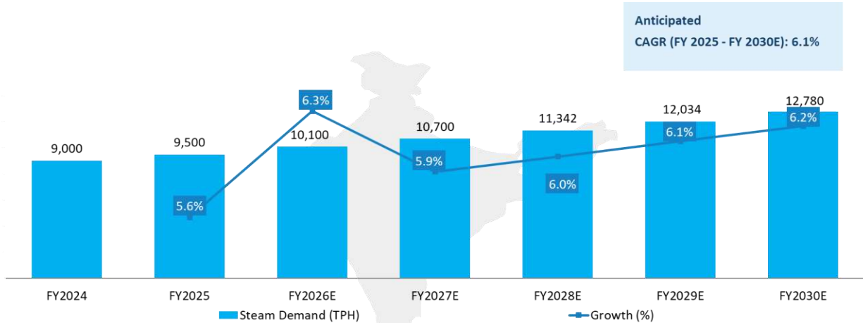
Exhibit 5.6: Process steam demand of Paper and Pulp industry, in TPH, India, FY2024 to FY2030E
